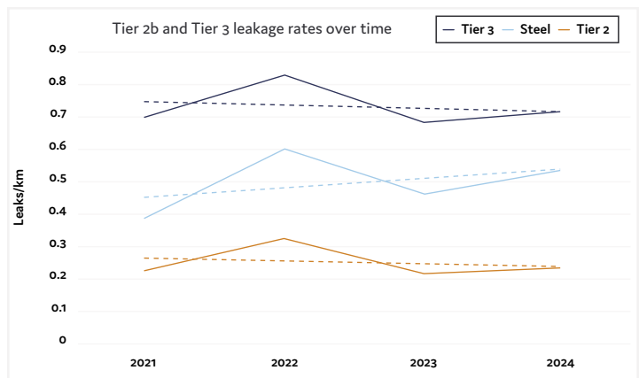
Figure 6.3 Tier 2b and Tier 3 leakage rates over time
