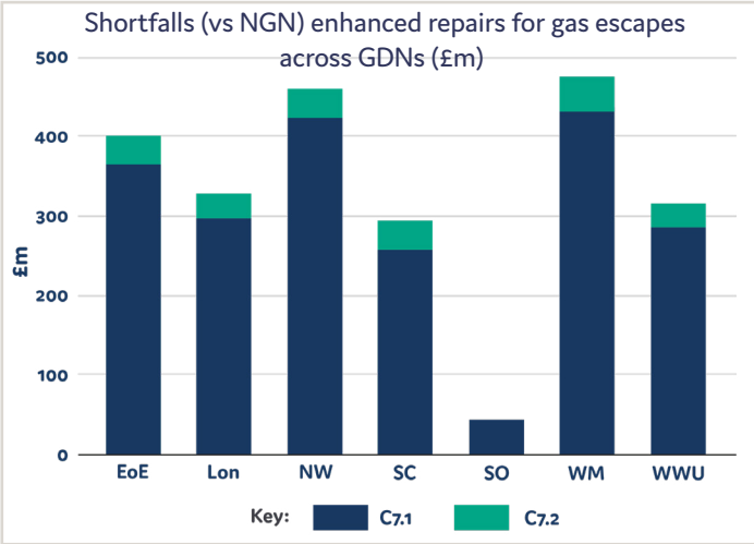
Figure 3.2 Shortfalls (vs NGN) enhanced repairs for gas escapes across GDNs (£m)
