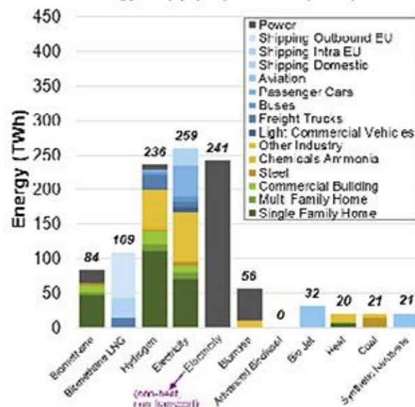
Energy Supply by Source (TWh)
