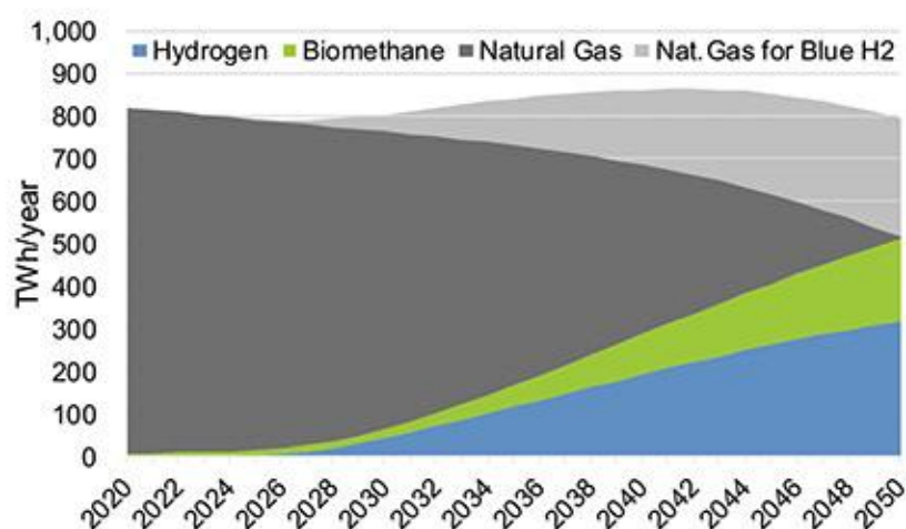
Figure 11 Network gas quantities along the Pathway 56
