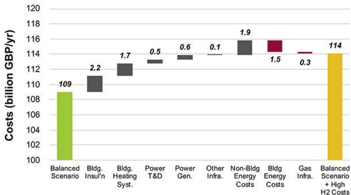
Figure 25 Impact of more costly hydrogen on 2050 energy system cost
