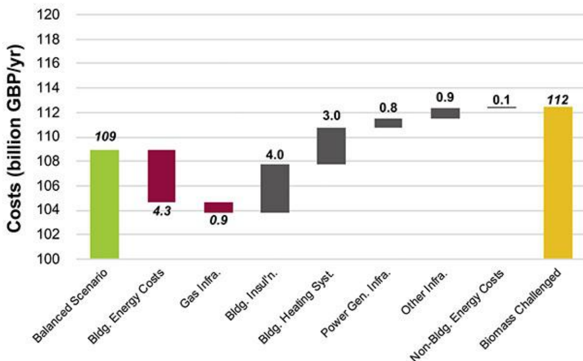
Figure 24 Impact of less biomass imports on 2050 energy system cost
