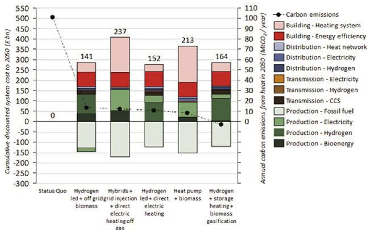
Figure 37 Uncertainty in cumulative additional system cost to 2050 – Mixed scenarios (Figure 1-6 in study)
