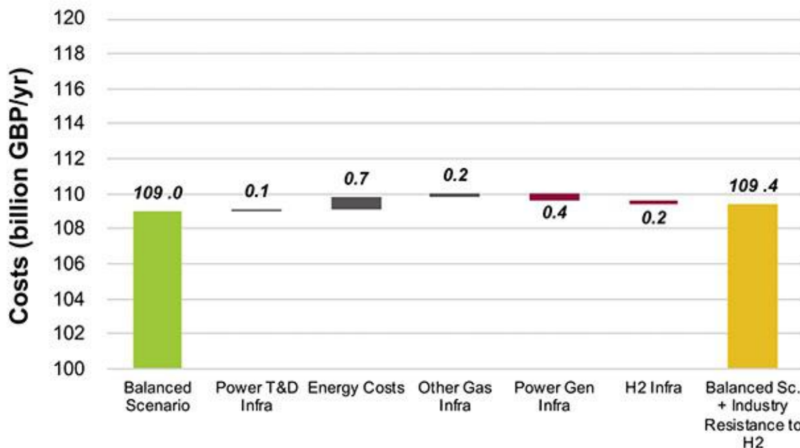
Figure 26 Impact of industry resistance to hydrogen on 2050 energy system cost
